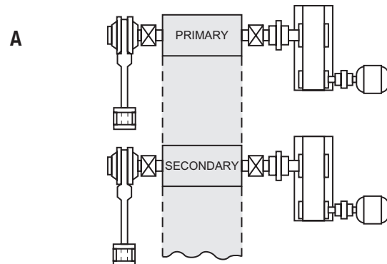
Figure 5 — Dual motor, dual backstop, dual pulley arrangement – Refer to the Rexnord factory for selection.
