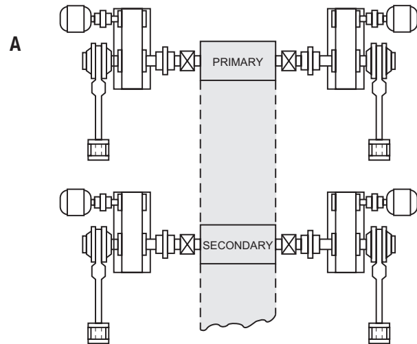
Figure 4 — Tandem motor, tandem backstop, dual pulley arrangement – Refer to the Rexnord factory for selection.
