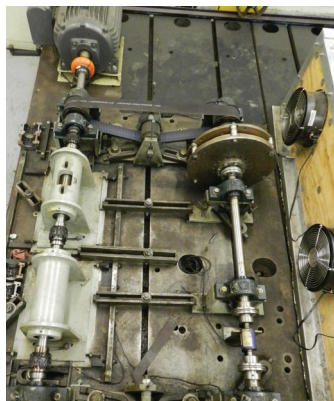
Operating under misalignment test stand
